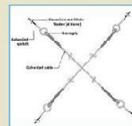
Cable Bracing
